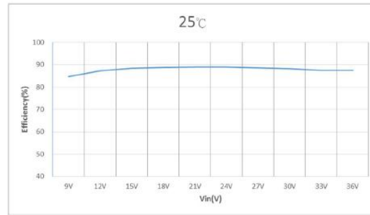
Figure 2 : Efficiency VS. Input Voltages at 100% rated power
